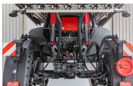
Slide axles that are arranged one after the other and hydropneumatic suspension
